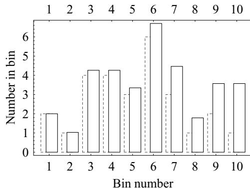
Fig. 7.10. Distribution of spectral indices (optical to X-ray) for a sample of optically selected quasars, showing the observed distribution (dashed boxes) and the estimated true distribution (solid boxes) after including the lower limits.
