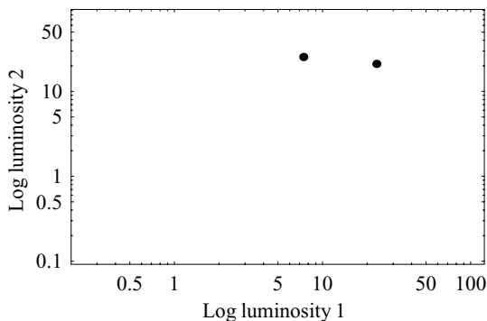
Fig. 7.6. Results of a simulation of a flux-limited survey of galaxies, where each galaxy has two statistically independent luminosities associated with it.
