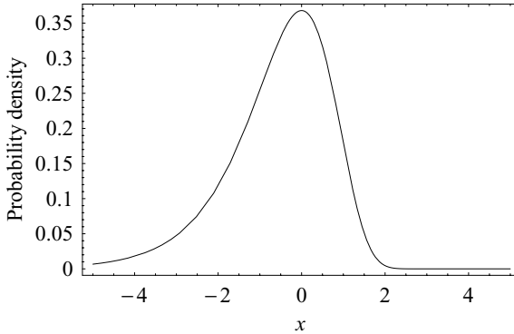
Fig. 3.2. The probability distribution of the logarithm of data drawn from an exponential distribution.
