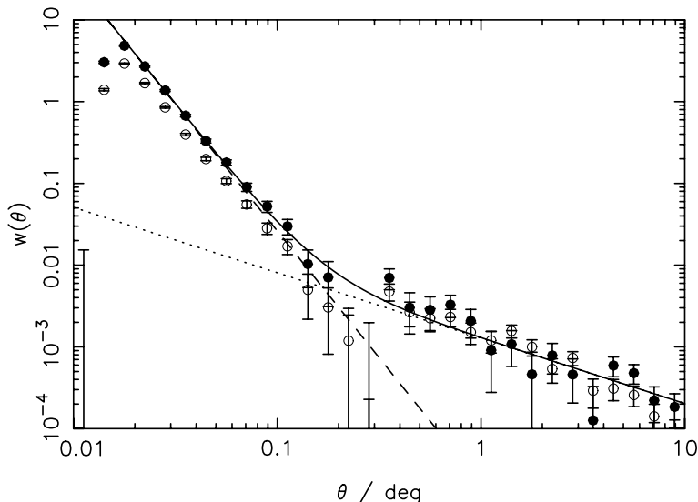
Fig. 9.3. The angular correlation function w(\theta) for the source catalogue of the NVSS survey, at S_{1.4\text{GHz}} = 20 mJy (solid circles) and 10 mJy (open circles). The best-fitting sum of two power laws for the 20 mJy data is shown as the solid line, with the two power laws shown individually, dashed due to multiple-component sources, dotted due to galaxy clustering.
