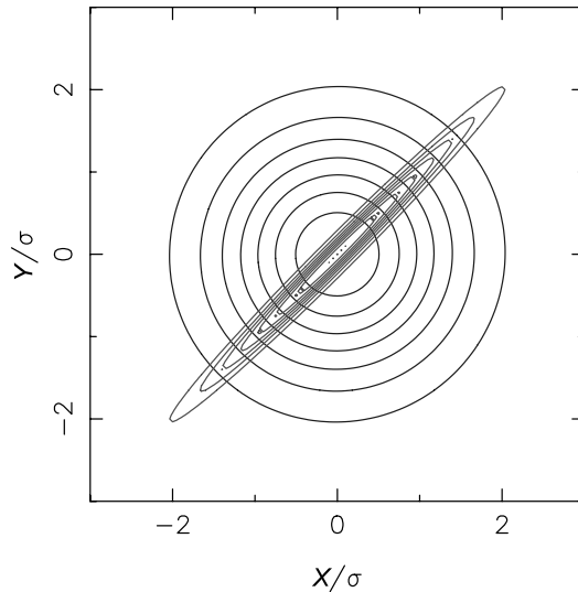
Fig. 4.4. Linear contours of the bivariate Gaussian probability distribution; the near-circular contours represent \rho = 0.01 , a bivariate distribution with little connection between x and y , while the highly elliptical contours represent \rho = 0.99 , indicative of a strong correlation between x and y . Negative values of \rho reverse the tilt, and indicate what is loosely referred to as anticorrelation.
