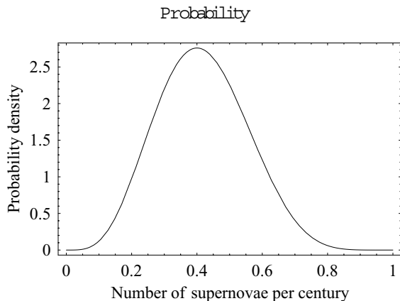
Fig. 2.3. The posterior probability distribution for \rho , given that we have four supernovae in ten centuries.
