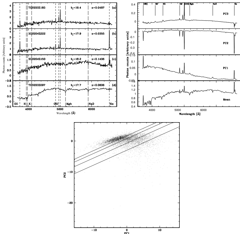
Fig. 4.9. Top left: examples of 2dF spectra prepared for PCA. Instrumental and atmospheric features have been removed, with the spectra transformed to the rest frame, resampled to 4\text{\AA} bins and normalized to unit mean flux. Top right: the mean spectrum and first three principal components; the sign of the PCs is arbitrary. Below: distribution of 2dF galaxy spectra in the PC1–PC2 plane. Slanted lines divide the plane into the five spectral classes adopted by Folkes et al.
