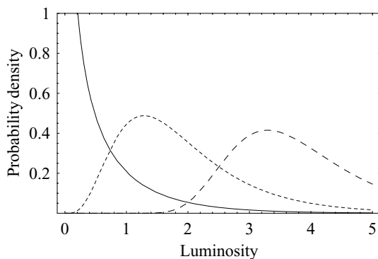
Fig. 3.5. The Schechter luminosity function (solid curve) and the distribution of the maximum of 10 and 100 samples from the distribution, plotted as short- and long-dash curves respectively.
