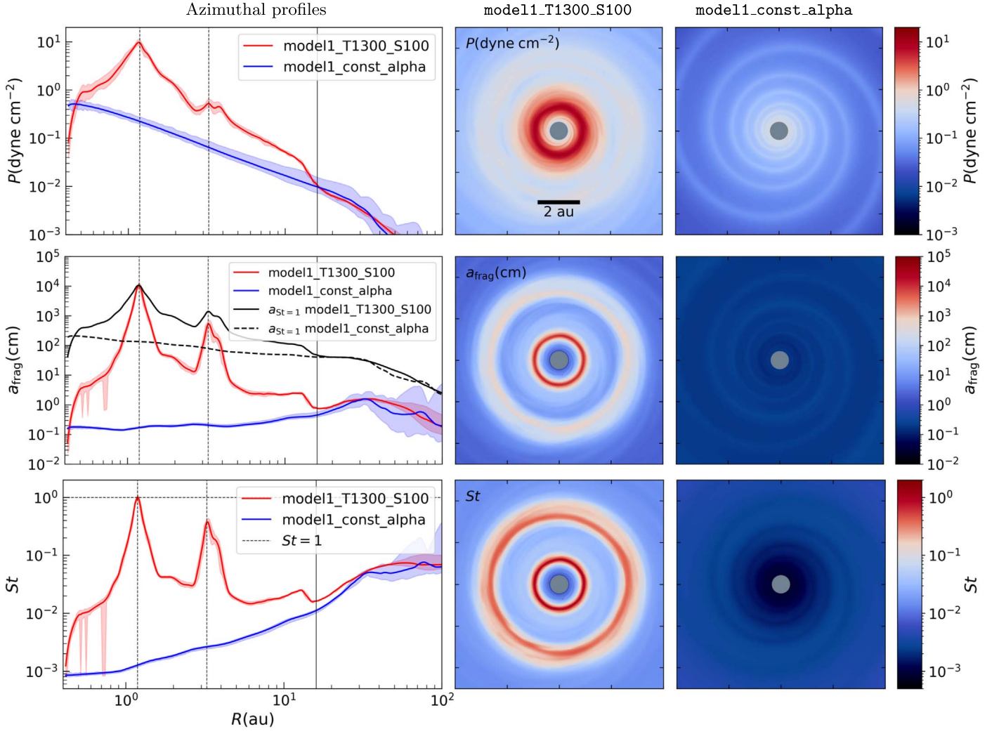
Figure 8. Typical inner disk structure of both fiducial models shown at 0.35 Myr, with respect to quantities that are relevant for planet formation—vertically integrated pressure, dust grain fragmentation radius (along with the grain size at Stokes number unity), and Stokes number at the dust grain fragmentation radius. Left: profiles of the azimuthally averaged parameters, with the shaded area showing the extent between the maximum and the minimum value at the given radius. The two vertical dashed lines mark the location of the two rings, while the solid line marks the outer extent of the dead zone. Right: distribution of the same parameters plotted in the inner 10 \times 10 au box.
