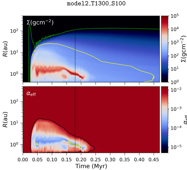
Figure 12. Spacetime plots for model12_T1300_S100, showing effects of a smaller cloud core mass on the evolution of gas surface density and \alpha_{\text{eff}} . The green contour in the top panel corresponds to \Sigma = 1 \text{ g cm}^{-2} and the yellow contour to \Sigma = \Sigma_a = 100 \text{ g cm}^{-2} . The black contour in the bottom panel shows the extent of the dead zone, while the yellow contour corresponds to \alpha_{\text{eff}} = 10^{-4} . The vertical dashed lines show the time corresponding to the azimuthal profiles in Figure 9.
