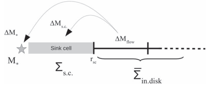
Figure 1. Schematic illustration of the inner inflow–outflow boundary condition. The mass of material \Delta M_{\text{flow}} that passes to the sink cell from the active inner disk is further divided into two parts: the mass \Delta M_* contributing to the growing central star, and the mass \Delta M_{\text{s.c.}} settling in the sink cell. r_{\text{sc}} is the radial position of the sink–disk interface, set equal to 0.4 au.
