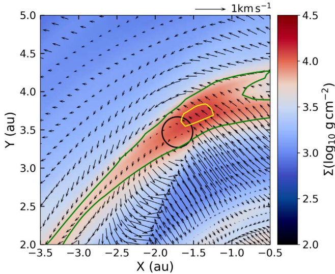
Figure 6. Velocity field superimposed on the gas surface density distribution, showing formation of a vortex near the outer ring. The black circle marks the region of the vortex, while the green and yellow contour lines show the onset of GI with Q = 2 and 1 levels, respectively.
