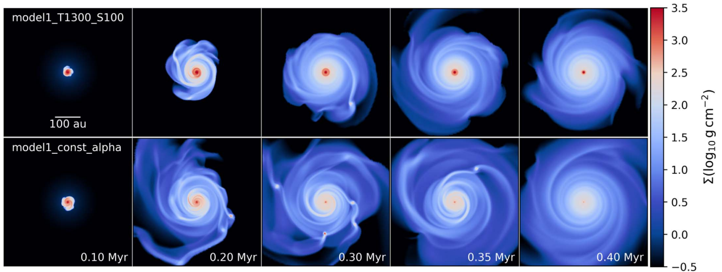
Figure 2. Evolution of the disk gas surface density distribution for the fiducial layered disk model (model1_T1300_S100; top row) and fiducial fully MRI-active model (model1_const_alpha; bottom row) over a region of 500 \times 500 au. Note that the former consistently shows a higher surface density in the central regions, while the latter shows a larger viscous spread of the disk.
