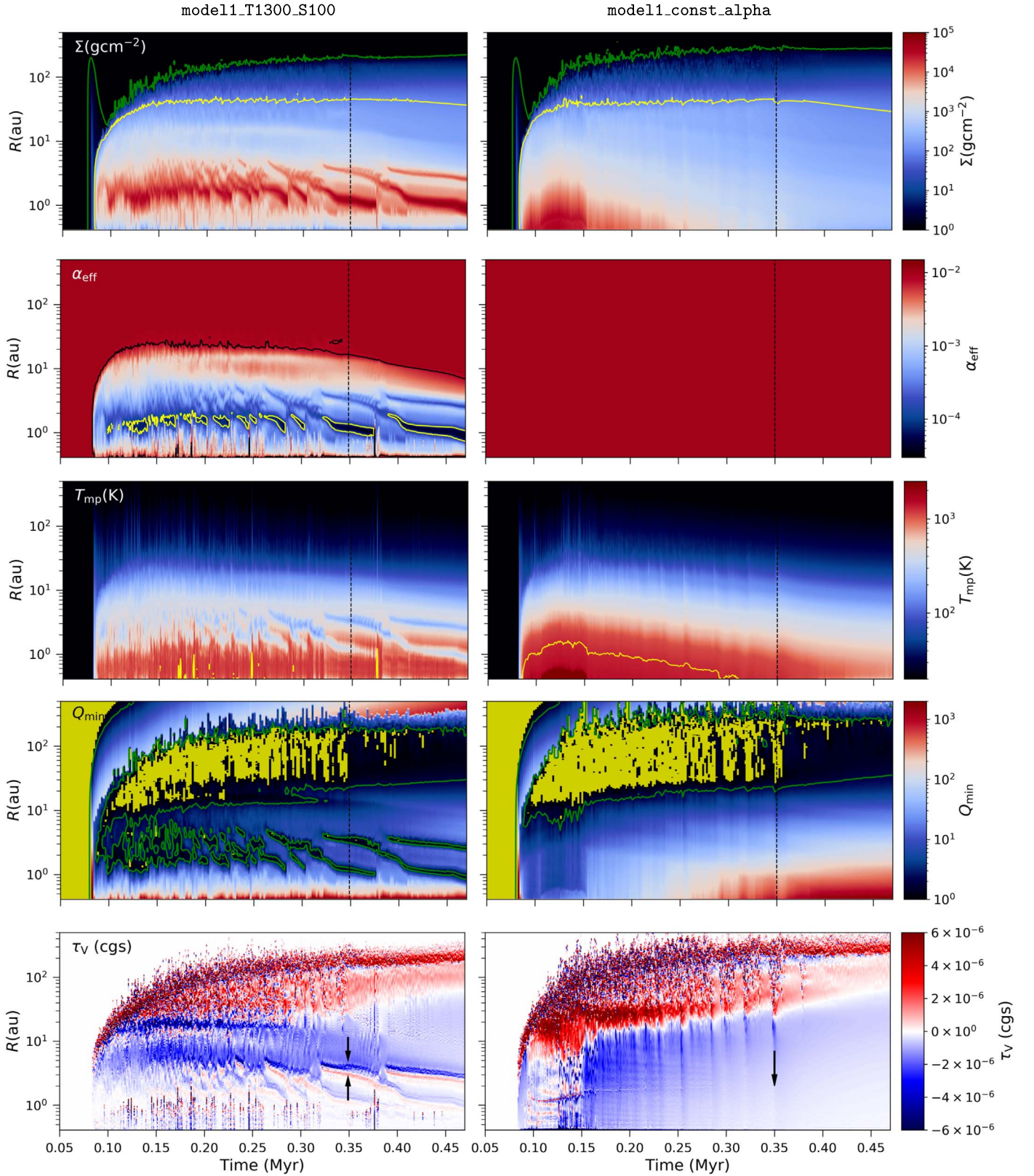
Figure 4. Spacetime plots for the two fiducial models, with the rows depicting the evolution of azimuthally averaged quantities \Sigma , \alpha_{\text{eff}} , and T_{\text{mp}} , the minimum in Q -parameter, and viscous torque. The green and yellow curves in \Sigma show 1 and 100 \text{ g cm}^{-2} contours, respectively. The black contour in \alpha_{\text{eff}} shows the extent of the dead zone as defined in Section 3.1, while the yellow lines show the 10^{-4} contour. The yellow lines in the midplane temperature plots show T_{\text{crit}} = 1300 \text{ K} contours. The yellow shaded area in the Q -parameter plot shows the gravitationally unstable region where Q \leq 1 , while the green contours show the Q = 2 level. The layered disk model (first column) shows qualitatively different behavior with the formation of long-lived rings, which can be clearly seen as high surface density and low-viscosity bands. The vertical dashed lines show the time corresponding to the static images in Figure 3, while the arrows in the last row show the direction of viscous torques, which act toward building up of the rings in the layered disk.
