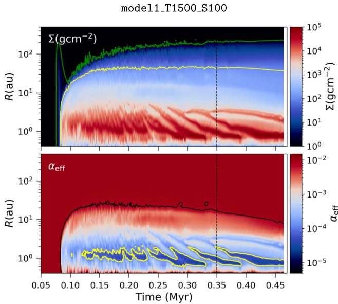
Figure 10. Spacetime plots for model11_T1500_S100 , showing effects of increasing T_{\text{crit}} to 1500 K on the evolution of gas surface density and \alpha_{\text{eff}} . The green contour in the top panel corresponds to \Sigma = 1 \text{ g cm}^{-2} and the yellow contour to \Sigma = \Sigma_a = 100 \text{ g cm}^{-2} . The black contour in the bottom panel shows the extent of the dead zone, while the yellow contour corresponds to \alpha_{\text{eff}} = 10^{-4} . The vertical dashed lines show the time corresponding to the azimuthal profiles in Figure 9.
