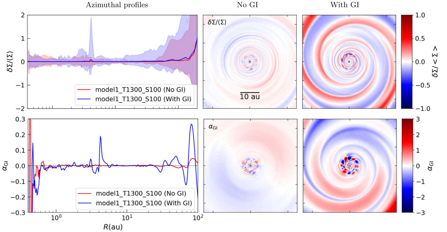
Figure 5. Fractional amplitude and \alpha_{\text{GI}} -parameter of the fiducial layered disk model when GI fragmentation (with Q < 1 ) was absent (0.350 Myr) compared to when it was present (0.326 Myr) in the rings. Left: profiles of the azimuthally averaged fractional amplitudes, with the shaded area showing the extent between the maximum and the minimum value at the given radius in the inner 100 au region. Right: distribution of the same parameter plotted in the inner 50 \times 50 au box.
