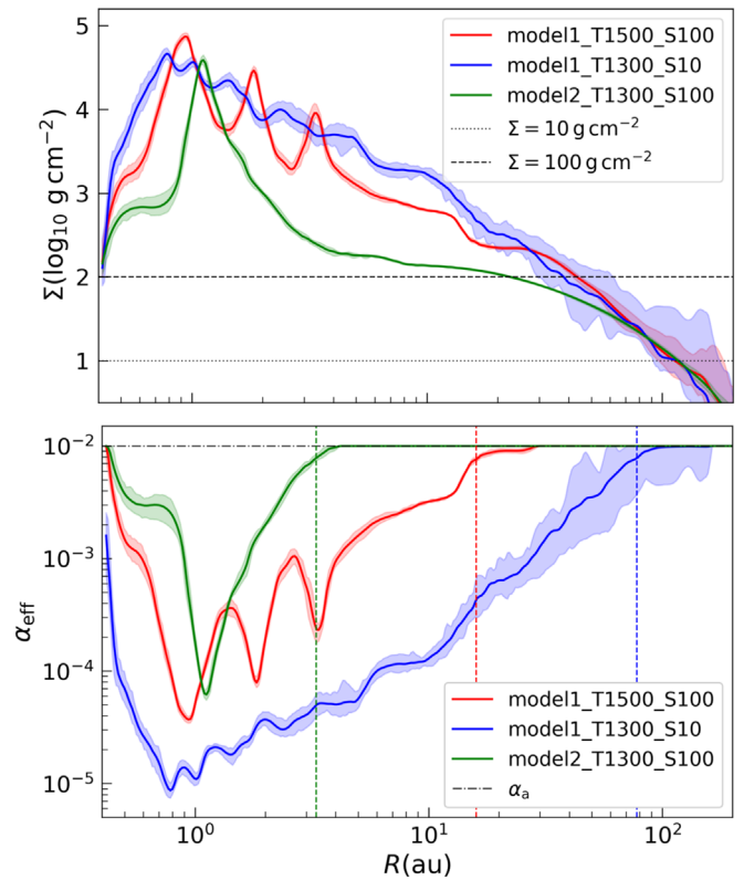
Figure 9. Typical inner disk structure of the fiducial adaptive alpha model compared to the variation of T_{\text{crit}} , \Sigma_a , and mass of the parent core with respect to the distribution of gas surface density and \alpha_{\text{eff}} in the inner 200 au region. The solid lines show azimuthally averaged quantities, with the shaded area showing the extent between the maximum and the minimum value at the given radius. The color-coded vertical dashed lines in the bottom panel show the outer extent of the dead zone for the respective model.
