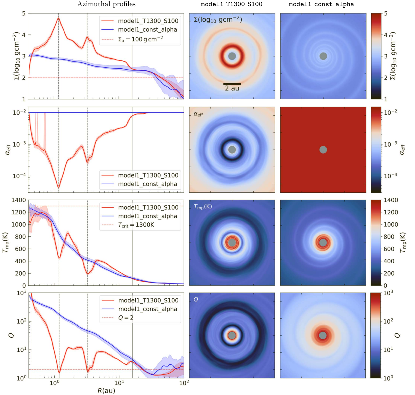
Figure 3. Typical inner disk structure of the fiducial layered disk model compared against that of the fully MRI-active disk model at 0.35 Myr, with respect to quantities—gas surface density, \alpha_{\text{eff}} , midplane temperature, and Toomre’s Q -parameter. Left: profiles of the azimuthally averaged parameters, with the shaded area showing the extent between the maximum and the minimum value at the given radius in the inner 100 au region. The two vertical dashed lines mark the location of the two rings, while the solid line marks the outer extent of the dead zone. Right: distribution of the same parameters plotted in the inner 10 \times 10 au box.
